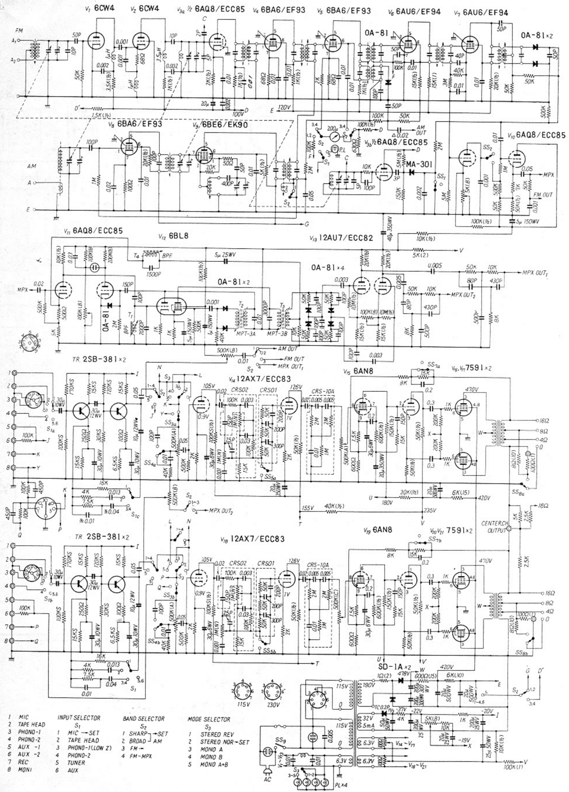
SANSUI MODEL 1000A FM STEREO RECEIVER
